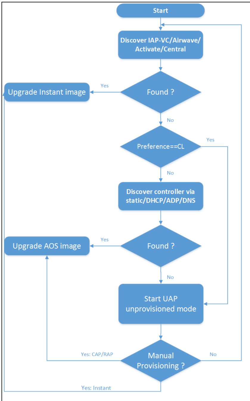
Figure 83 AP Discovery Logic
