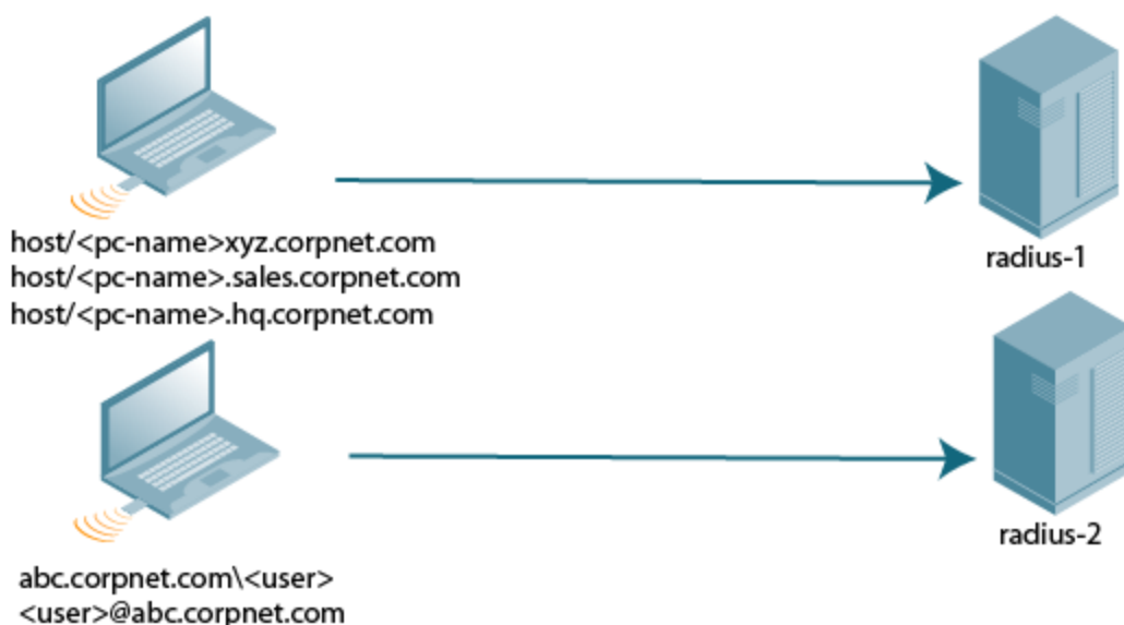
Figure 28 Domain-Based Server Selection Example
