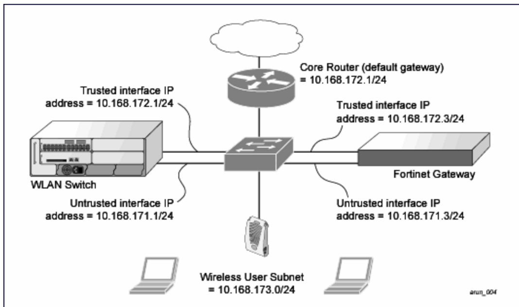
Figure 127 Example Route-Mode Topology
