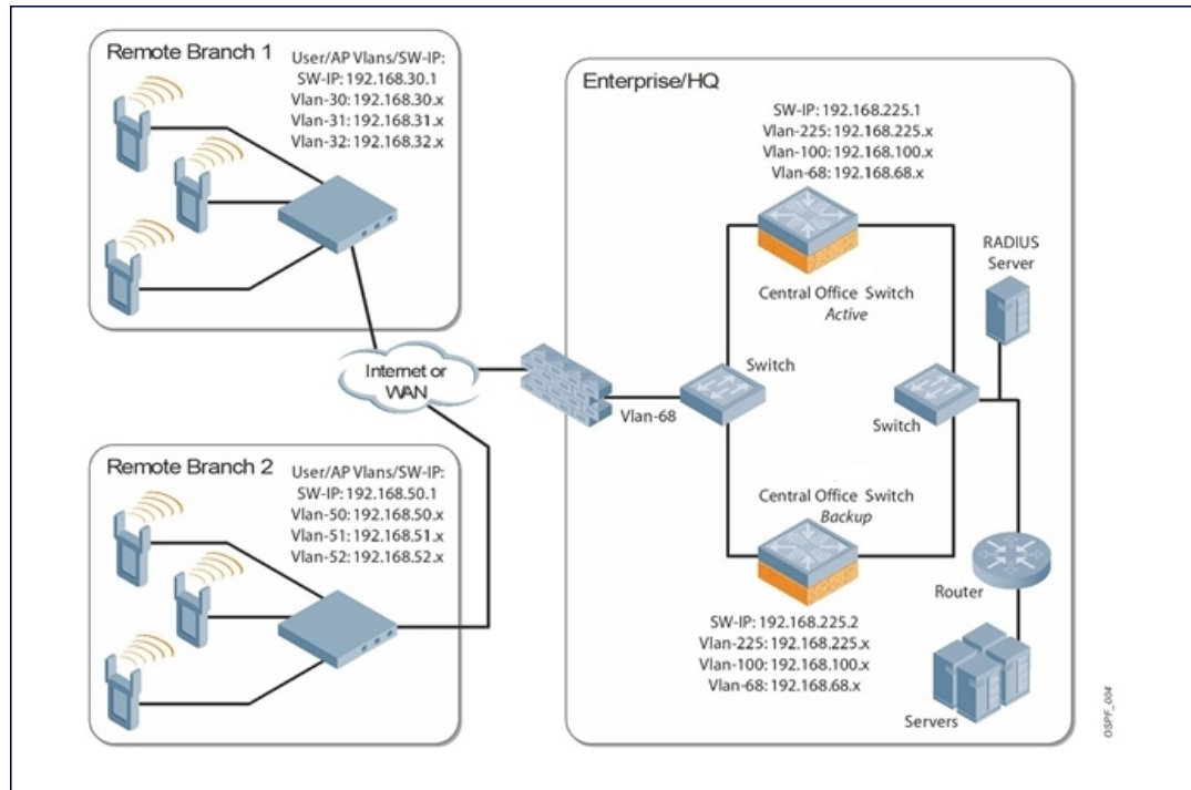
Figure 20 Sample OSPF Topology
