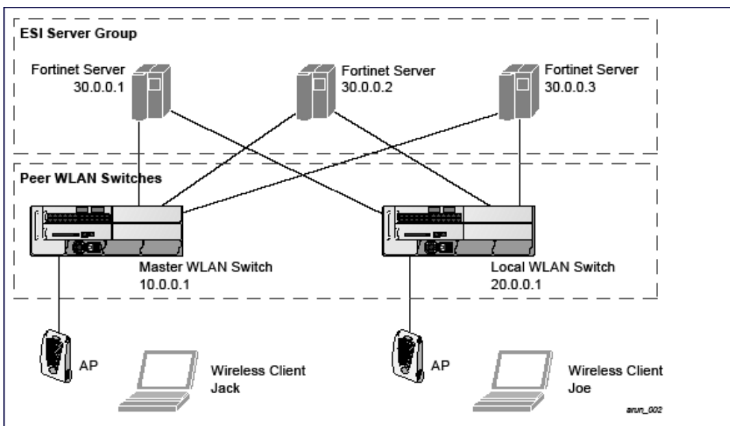
Figure 126 Peer managed device
